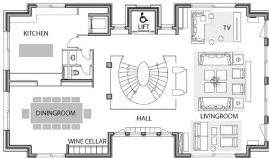
LEVEL 3 - Reception Surface = 200m 2
