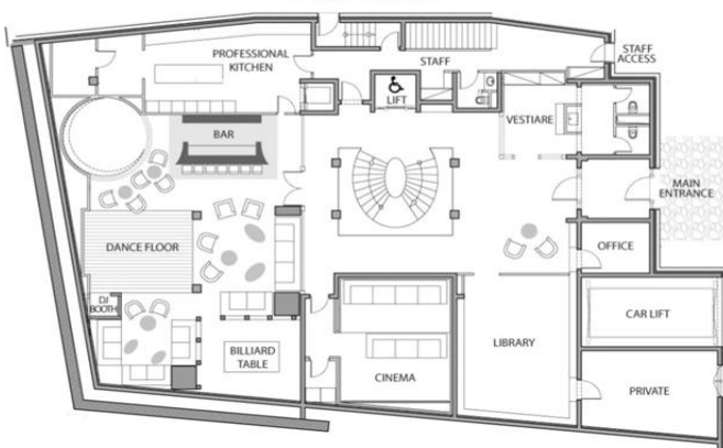
LEVEL 0 - Entrance
